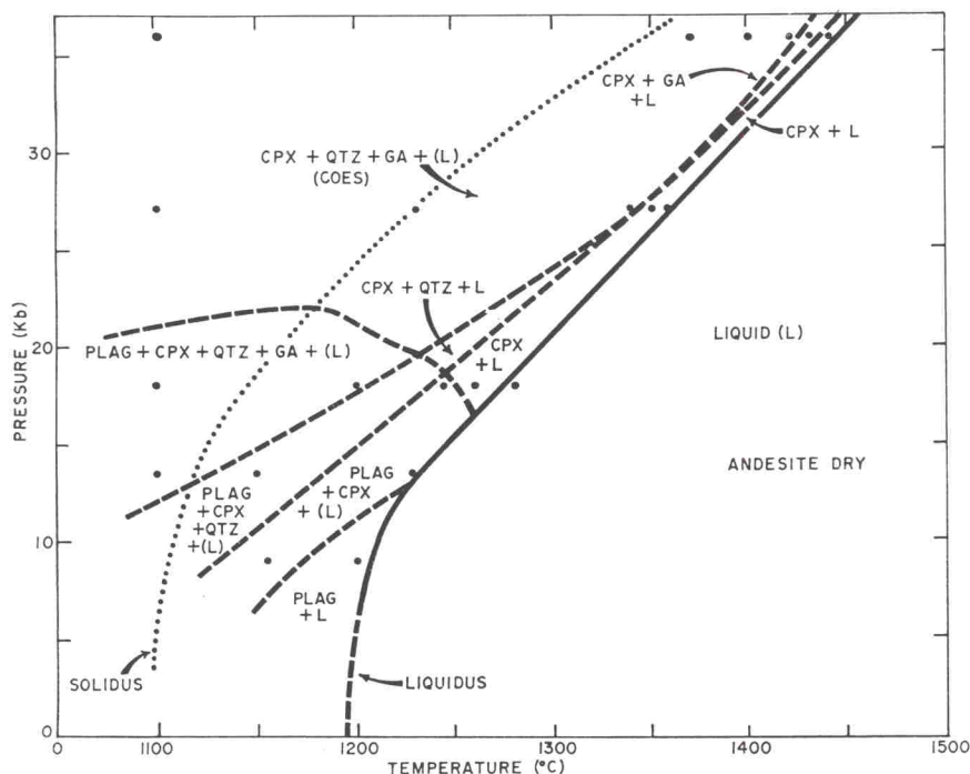
Fig. 1. P, T diagram for crystallization of andesite under anhydrous conditions (in this and subsequent P, T diagrams (1-4) solid points represent experimental runs, dashed lines the approximate phase boundaries, solid lines the liquidus and in Fig. 1 the dotted line denotes the approximate solidus. Abbreviations: L liquid; plag plagioclase; cpx clinopyroxene; qtz quartz; coes coesite; ga garnet; amph amphibole
